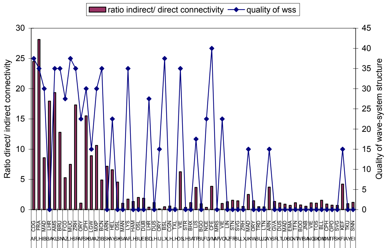
Figure 12. Ratio between weighted indirect connectivity and number of daily direct flights from the hub airport versus the presence and quality of the wave-system structure (40=very good; 35-37.5=good; 30-32.5=limited; 25-27.5=poor; 15-25=very poor; <15=absent)
