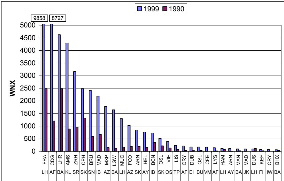
Figure 3. Number of weighted indirect connections (WNX) in 1990 and 1999 for the primary European airline hubs
